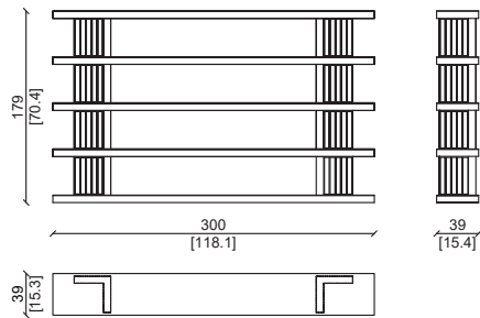
LIBRERIA LUXURY / LUXURY BOOKCASE
