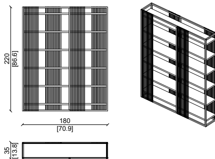
LIBRERIA/ BOOKSHELF
